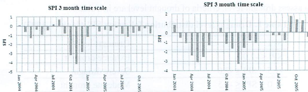
Figure 3. SPI 3 at Duc Xuyen (left) and Cau 14 (right)
