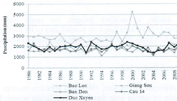
Figure 2. Annual average precipitation at monitoring stations
