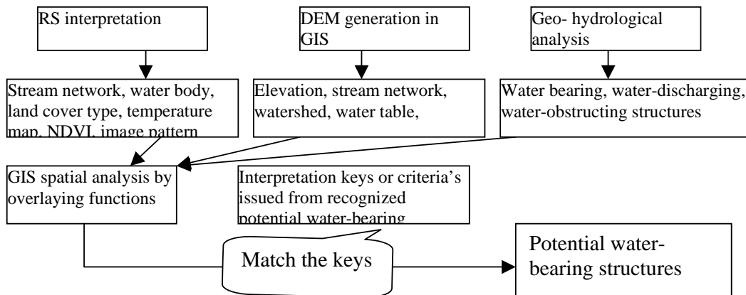
Figure 2. Modeling steps for hydrological analysis
