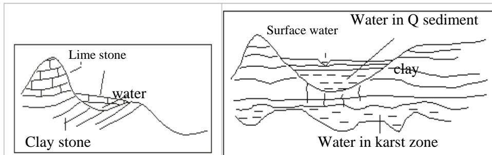
Figure 3. Water-holding valley (a), water-bearing trap structure (b)
