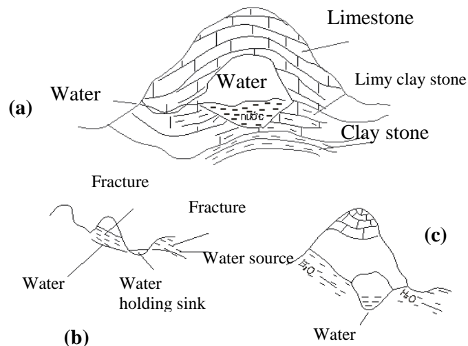
Figure 4. Perminian water bearing structure (a); water traps: opening (b) and ground (c)
