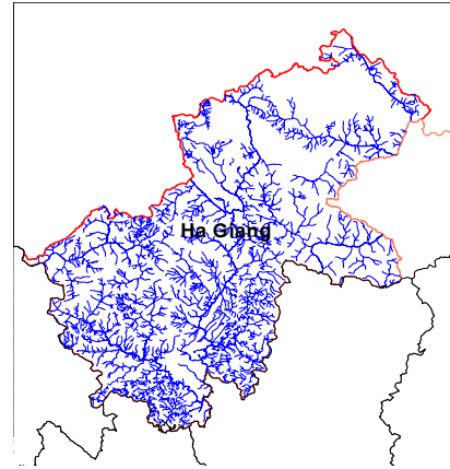
Figure 6. Stream network
