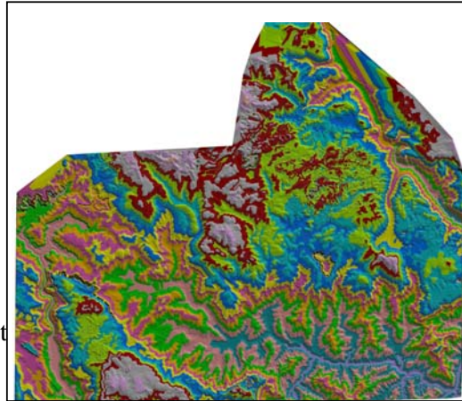
Figure 5. Lanform generated by GIS
