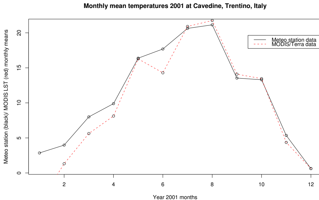
Figure 1: Comparison of monthly mean temperatures (2001) from Cavedine meteorological station (hourly data) and related MODIS/Terra data (max. two values per day).
