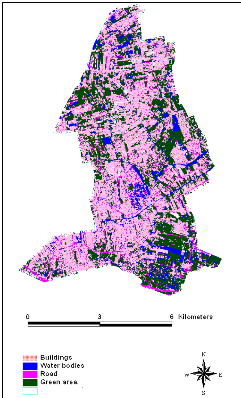
Figure 4. Classified map of the land cover types obtained from QuickBird image
